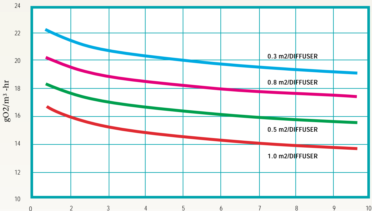
Oxygen transfer per m 3 and m submergence Efficiency depends on water depth, which is not reflected in this curve
